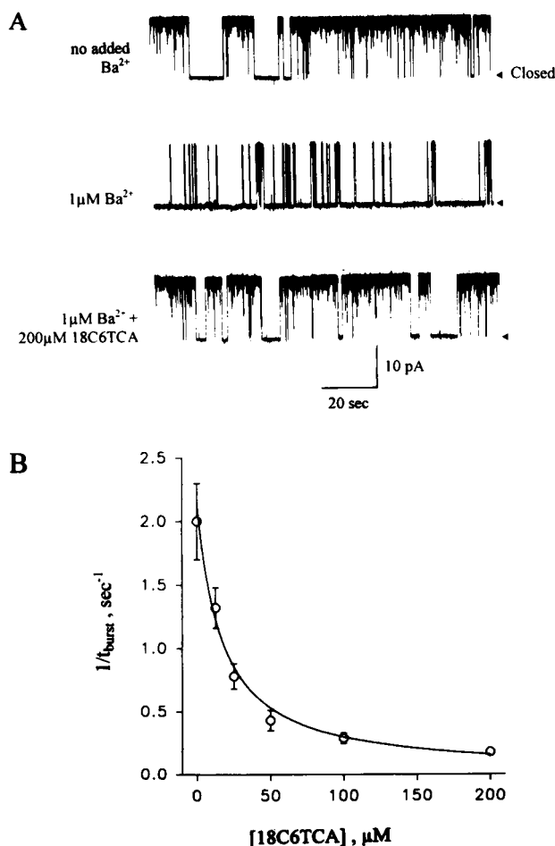
FIGURE 6 18C6TCA is a strong \text{Ba}^{2+} chelator. (A) Single-channel recordings of a highly activated BK channel ( \text{Ca}_i = 0.5\ \text{mM} ) successively bathed with the control internal solution, the same solution with 1\ \mu\text{M} \text{Ba}^{2+} added to the inner compartment, and finally, with the further addition of 200\ \mu\text{M} 18C6TCA. (B) The burst duration in the presence of 1\ \mu\text{M} \text{Ba}^{2+} was measured at different 18C6TCA concentrations. The inverse of the mean duration of the bursts separating \text{Ba}^{2+} blocking events (the \text{Ba}^{2+} blocking rate) is plotted as a function of the 18C6TCA concentration. The data points were fitted with Eq. 1.
