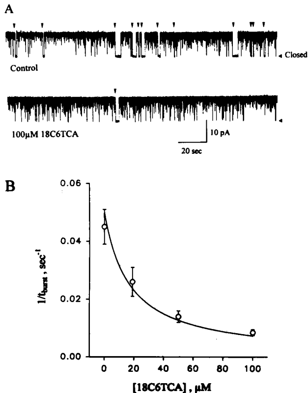
FIGURE 7 18C6TCA eliminates long shut events in fully activated BK channels. (A) Single-channel recordings of a BK channel in the presence of a high activating \text{Ca}_i concentration (0.5 mM) before and after addition of 100 \mu\text{M} 18C6TCA to the internal solution. Vertical arrowheads indicate shut events lasting more than 1 s. (B) Variation of the inverse of the mean duration of the bursts separating long shut events as a function of the 18C6TCA concentration. Data points were fitted with Eq. 1.
